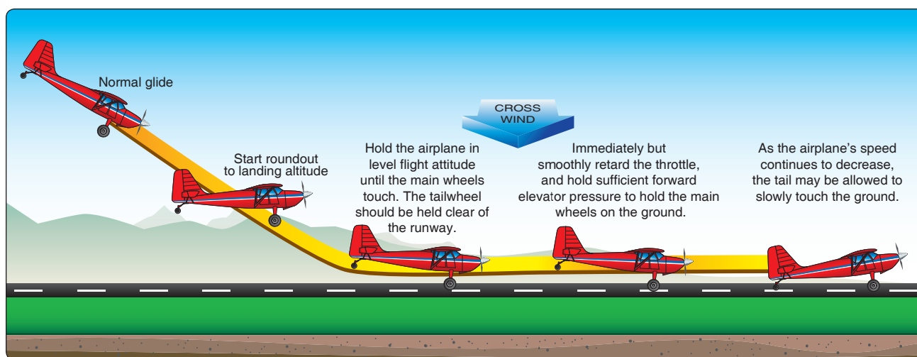
Figure 13-3. Wheel landing.
