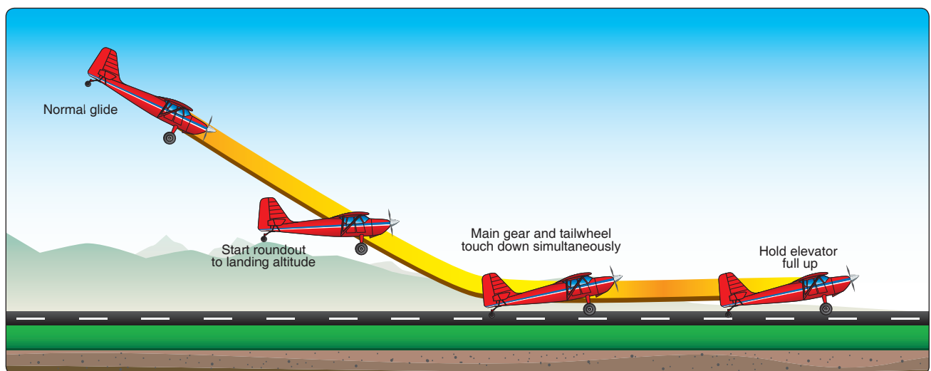
Figure 13-2. Tailwheel touchdown.
